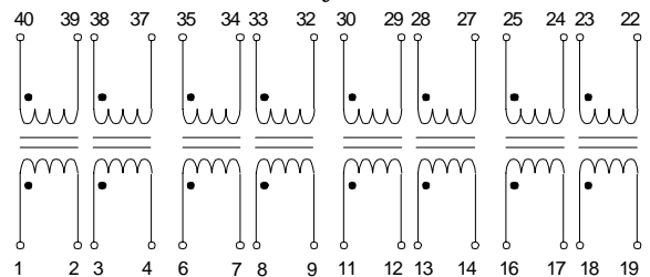
Schematic Style "40-6"
