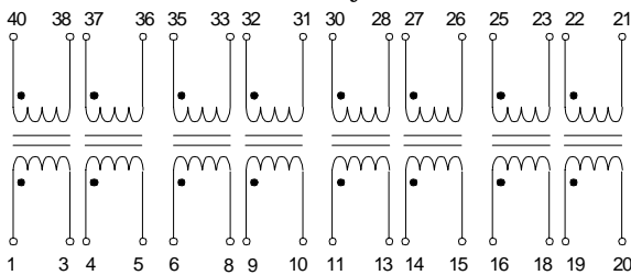
Schematic Style "40-5"
