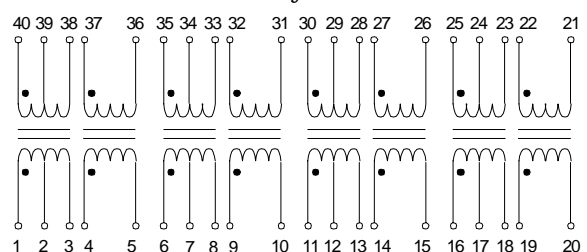
Schematic Style "40-8"
