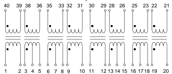
Schematic Style "40-4"
