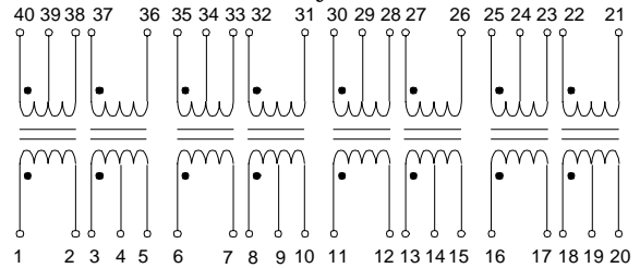
Schematic Style "40-2"
