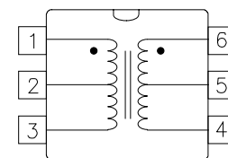
Schematic "C"
