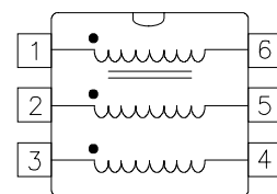
Schematic "A"
