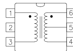
Schematic "D"
