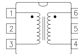
Schematic "B"
