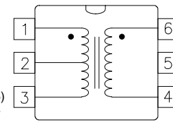
Schematic "E"
