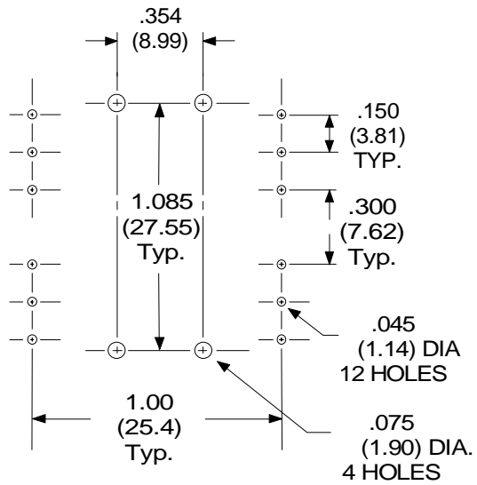
HOLE PATTERN COMP. SIDE
