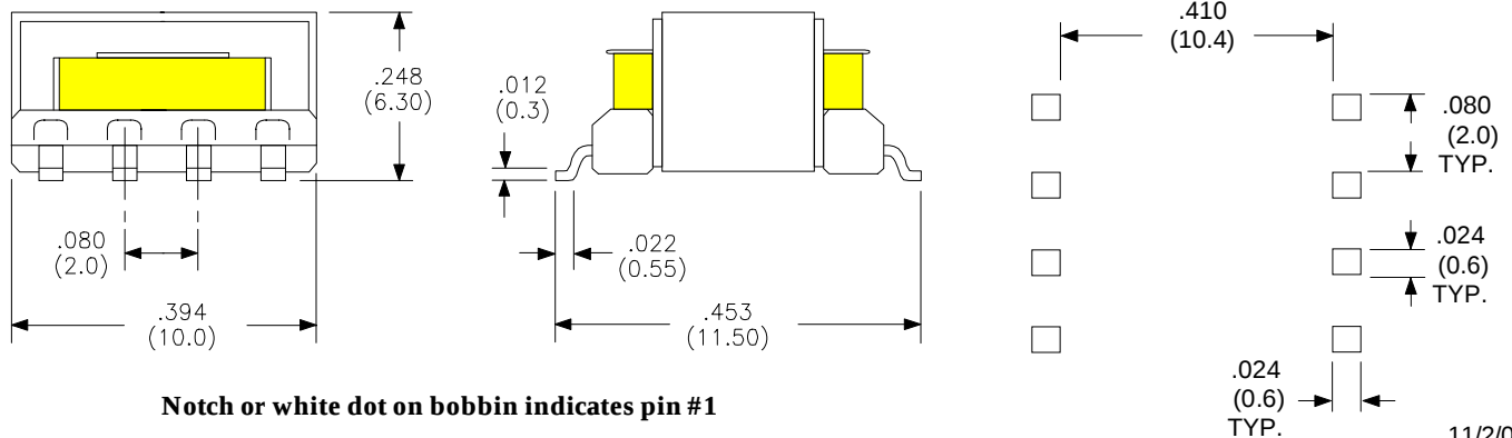
Physical Dimensions in inches (mm)
