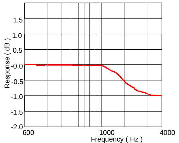
FREQUENCY RESPONSE
