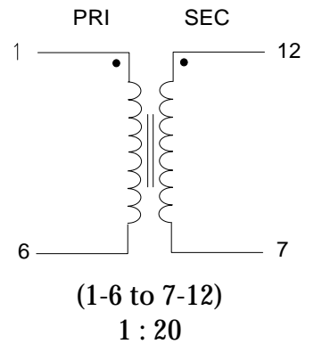
Schematic Diagram
