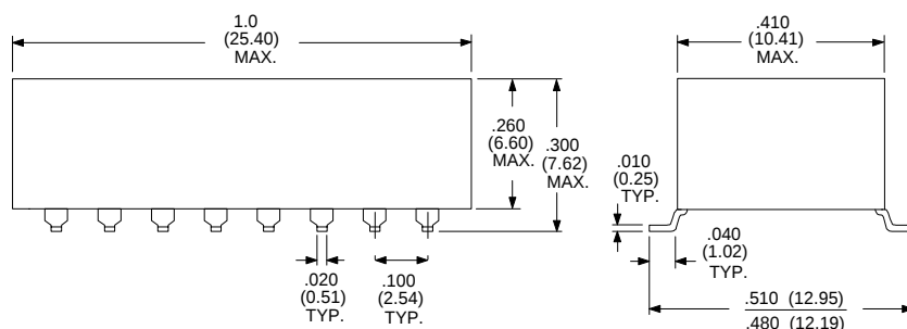
Dimensions in Inches (mm)
