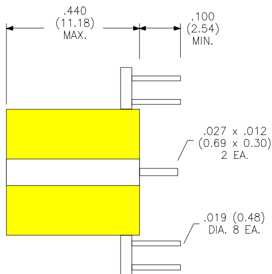
Physical Dimensions inches (mm)
