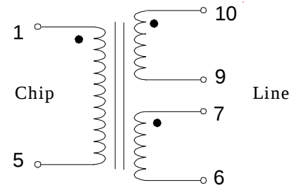
Schematic Diagram
