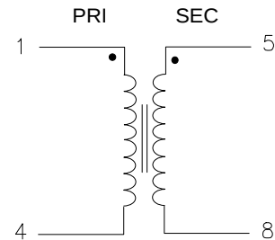
Schematic Diagram
