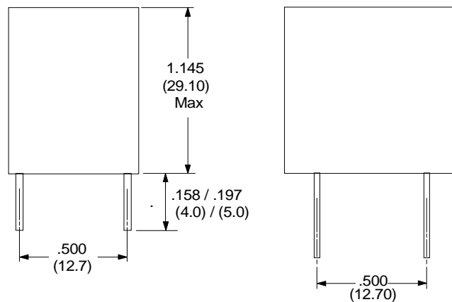
Physical Dimensions inches (mm)
