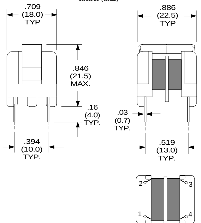
Physical Dimensions inches (mm)
