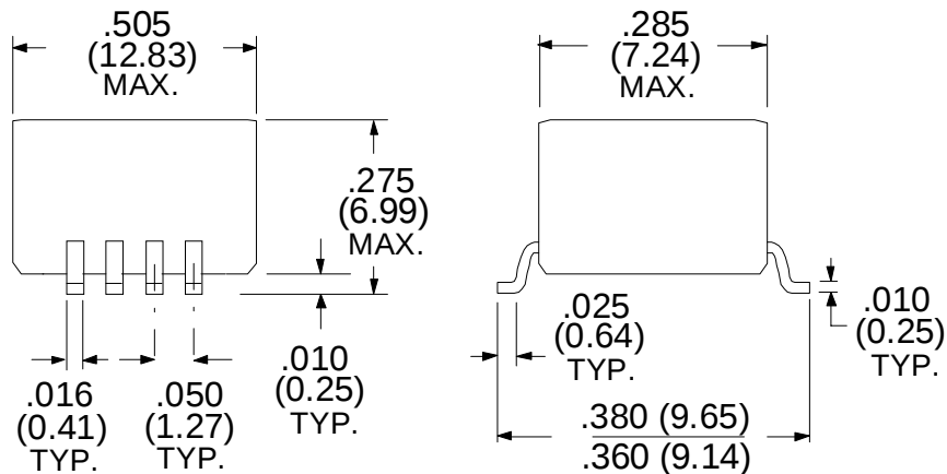
Physical Dimensions in inches (mm)
