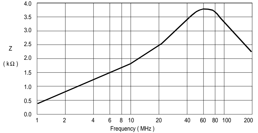
P/N F-1506 Typical Impedance Plot
