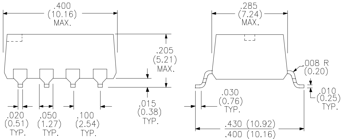
8 Pin Gull Wing Package Dimensions in inches (mm)
