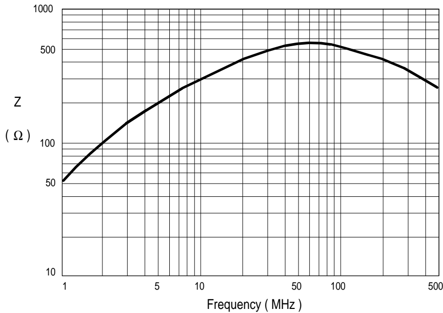
Typical Impedance Plot
